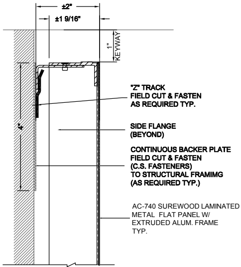
1 PERIMETER DETAIL (TOP) AC-740-FT1
