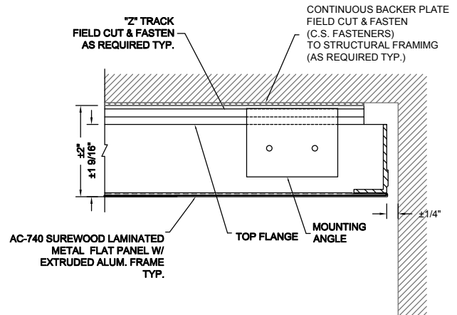
2 PANEL JOINT DETAIL AC-740-FS1
