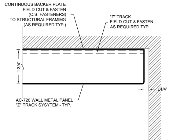
4 PERIMETER DETAIL (EDGE) AC-720-FE1
