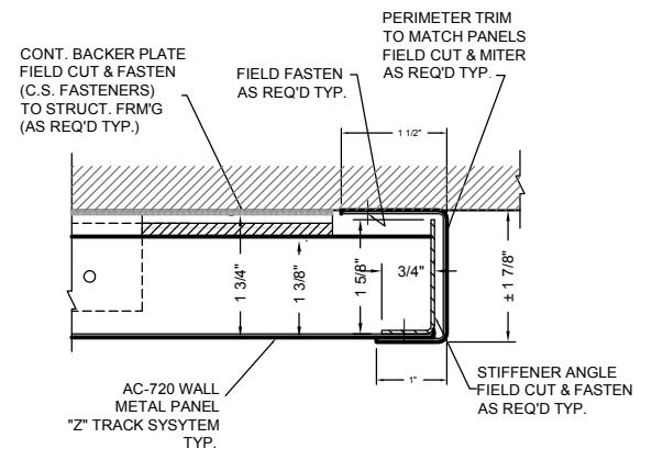
6 PERIMETER DETAIL AC-720-FCE1
