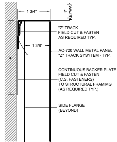
1 PERIMETER DETAIL (TOP) AC-720-FT1
