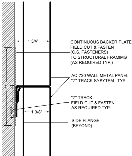
3 PANEL JOINT DETAIL AC-720-FM1
