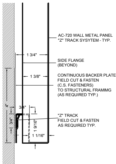
5 PERIMETER DETAIL (BASE) AC-720-FB1
