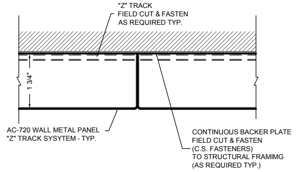
2 PANEL JOINT DETAIL AC-720-FS1
