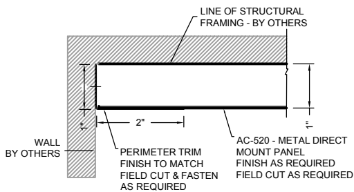
5 PERIMETER DETAIL AC-520-PFC2
