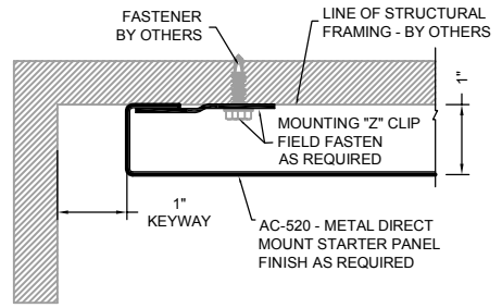
2 PERIMETER DETAIL AC-520-P1
