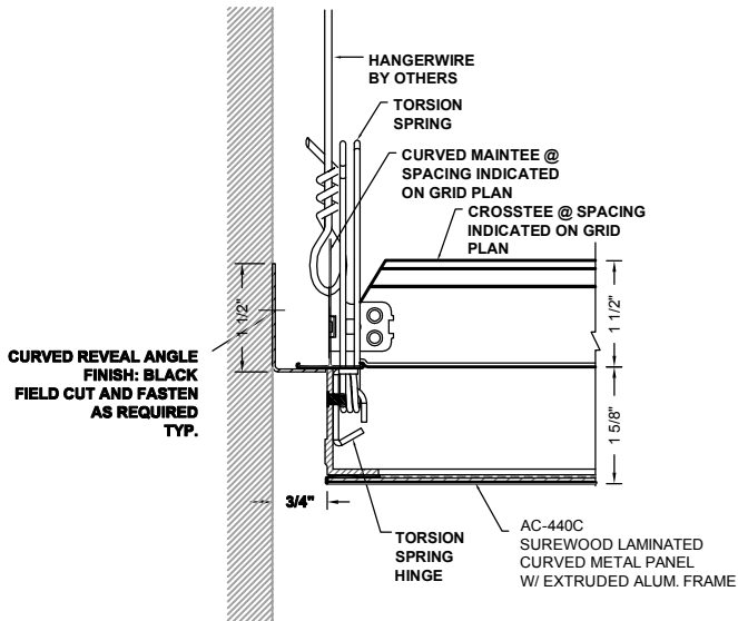
3 PERIMETER DETAIL AC-440C-P2
