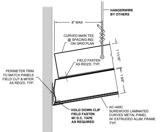
4 PERIMETER DETAIL AC-440C-PFC4
