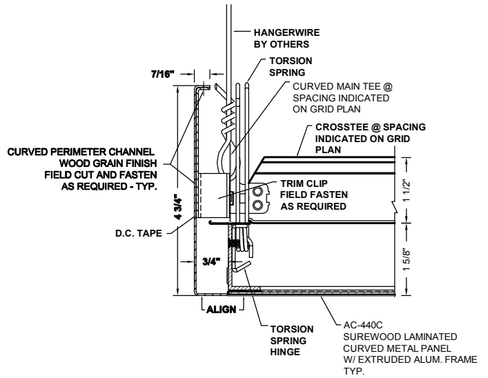
2 PERIMETER DETAIL AC-440C-P1
