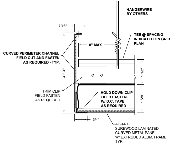
2 PERIMETER DETAIL AC-440C-PFC2
