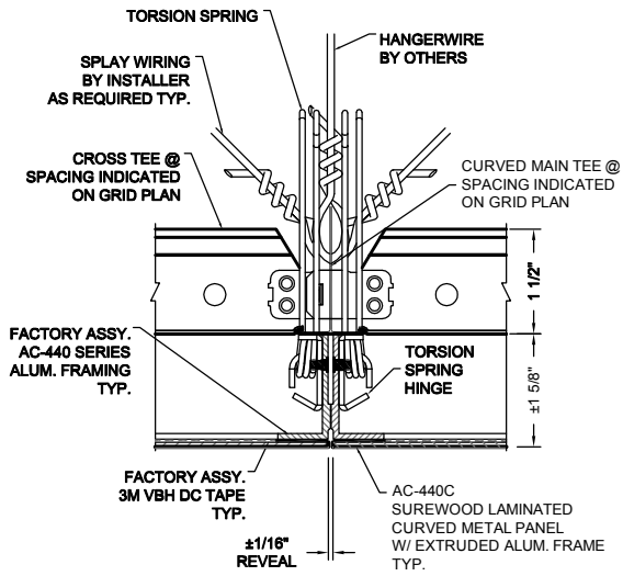
1 PANEL JOINT DETAIL AC-440C-PJ1
