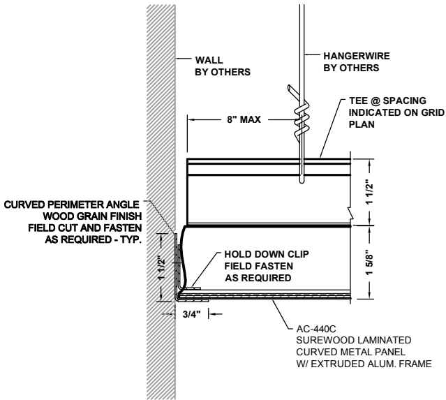
1 PERIMETER DETAIL AC-440C-PFC1
