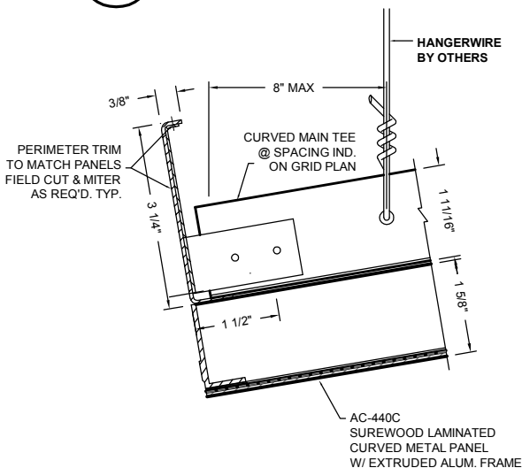
5 PERIMETER DETAIL AC-440C-P4
