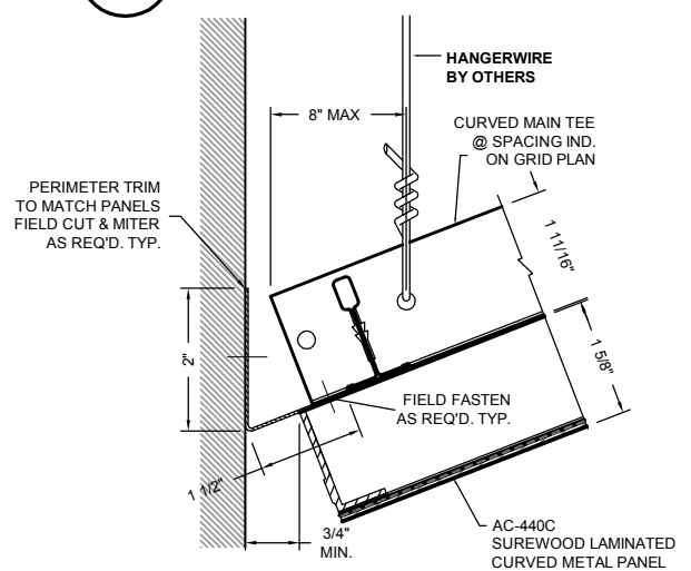
4 PERIMETER DETAIL AC-440C-P3
