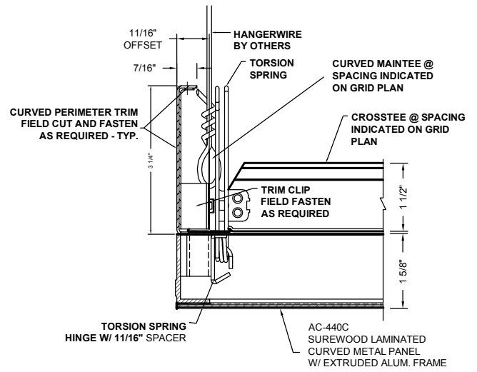
2 PERIMETER DETAIL AC-440C-P1
