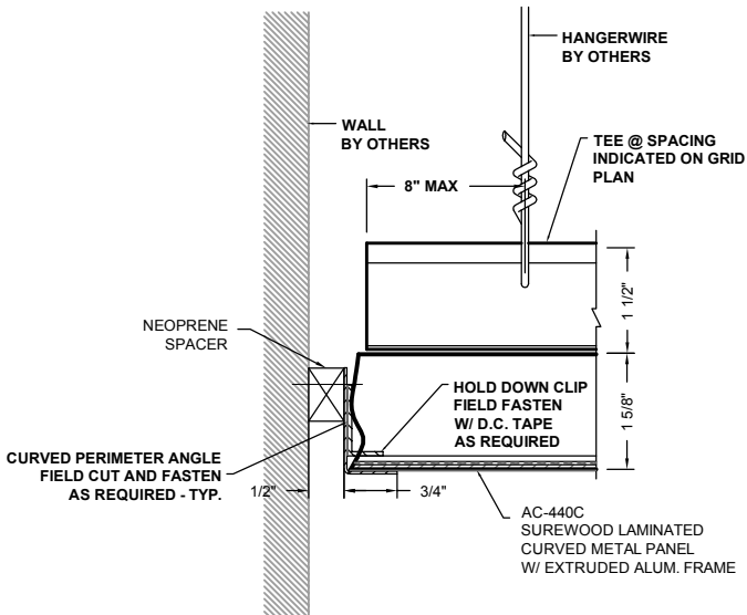
3 PERIMETER DETAIL AC-440C-PFC3
